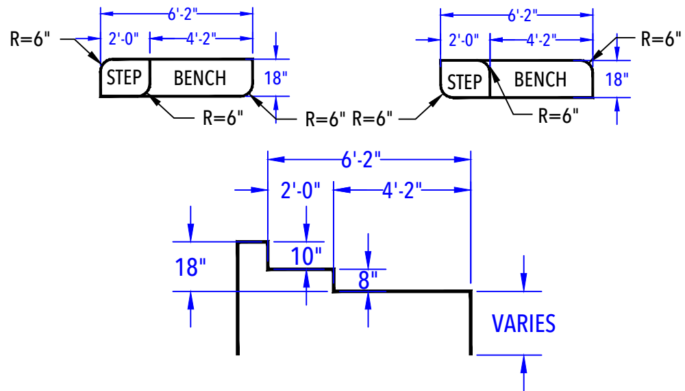
DEEP END BENCHES & STEP OUTS DETAIL (After Concrete & Liner) N.T.S.
