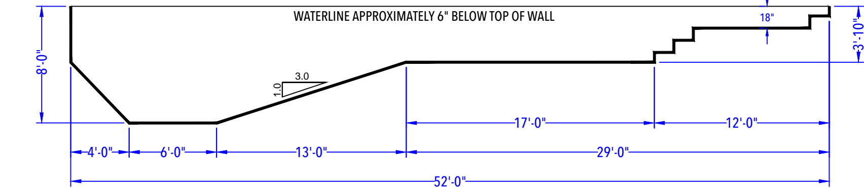
DEPTH DETAIL
