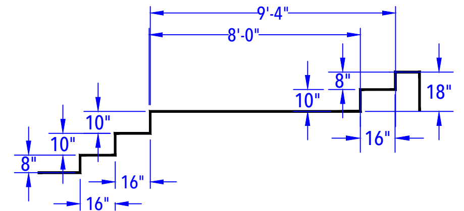
SUN DECK & STEP DETAIL (After Concrete & Liner) N.T.S.
