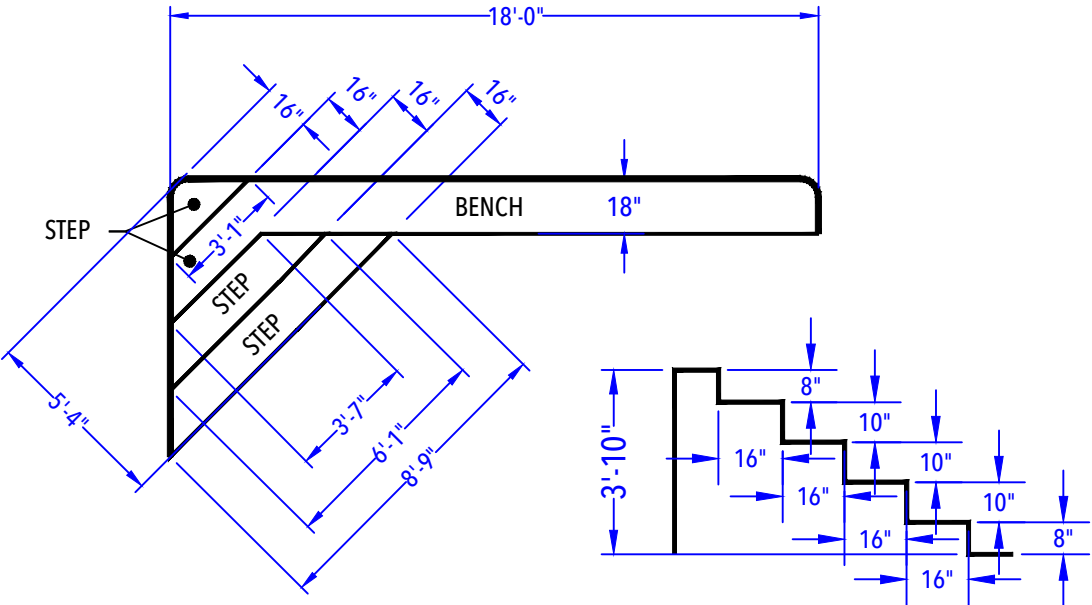
ENTRY STEP DETAIL (After Concrete & Liner) N.T.S.
