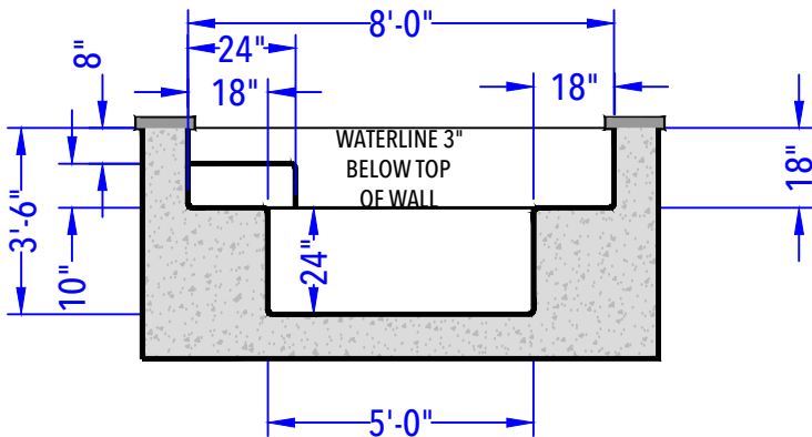
SPA PLAN & ELEVATION VIEW (After Concrete & Plaster)
