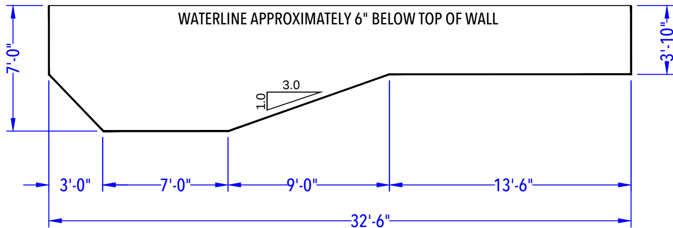
DEPTH DETAIL
