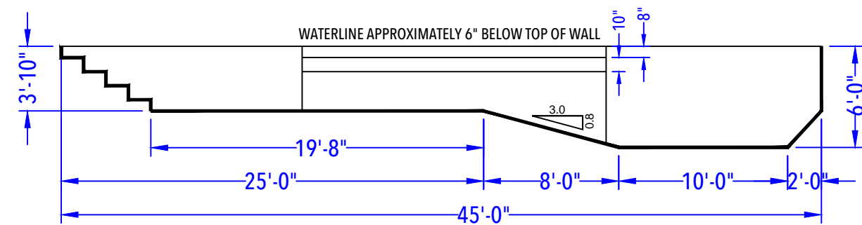
DEPTH DETAIL
