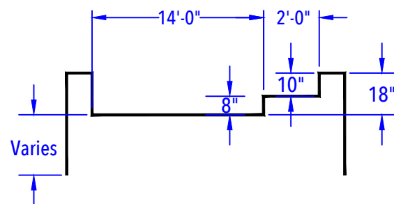
SIDE BENCH & STEP OUT DETAIL (After Concrete & Liner) N.T.S.
