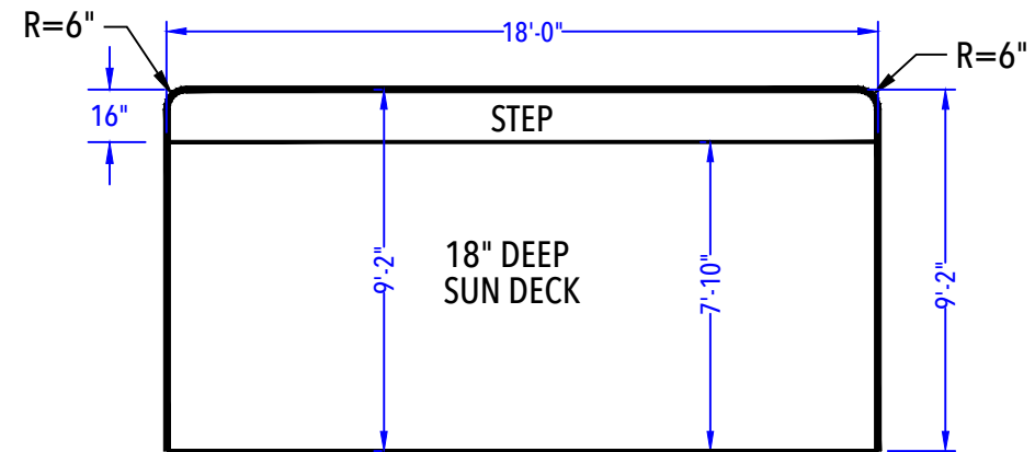
ENTRY STEP DETAIL (After Concrete & Liner) N.T.S.
