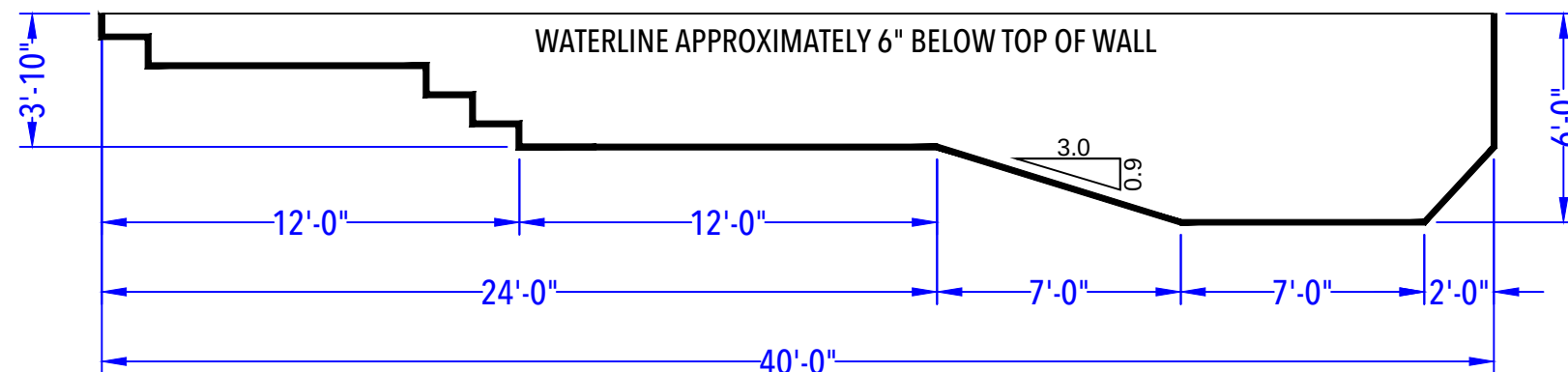
DEPTH DETAIL
