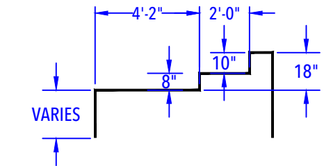
DEEP END BENCH & STEP OUT DETAIL (After Concrete & Liner)
