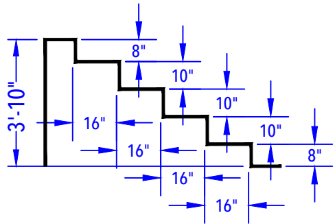
ENTRY STEP DETAIL (After Concrete & Liner)
