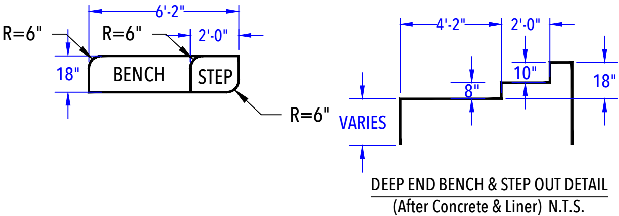
SIDE SUN DECK DETAIL (After Concrete & Liner) N.T.S.
