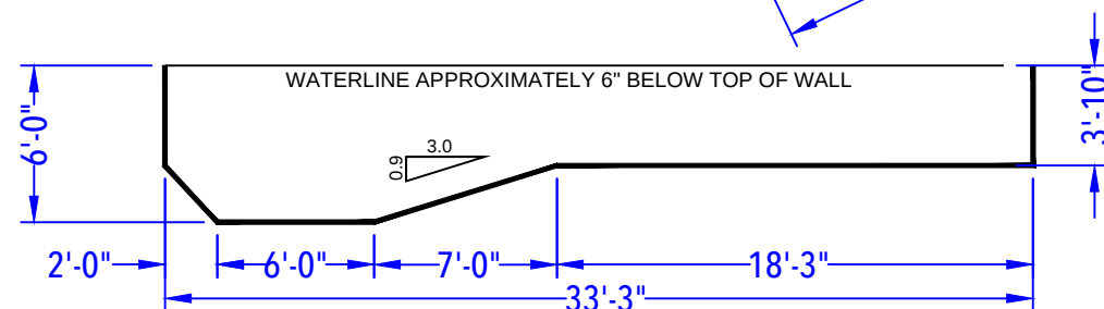
DEPTH DETAIL
