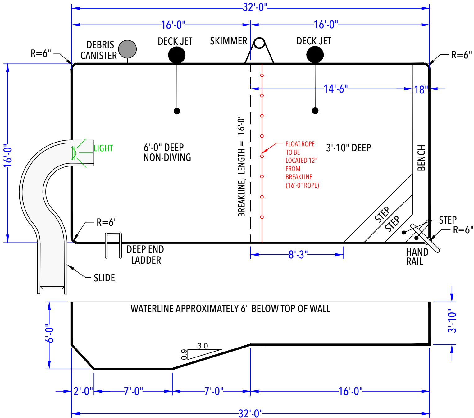
DEPTH DETAIL
