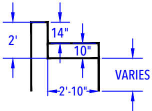
RADIUS DEEP END BENCH & STEP OUT DETAIL (After Concrete & Liner) N.T.S.
