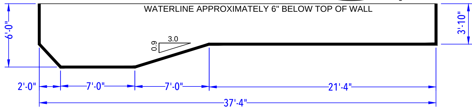
DEPTH DETAIL
