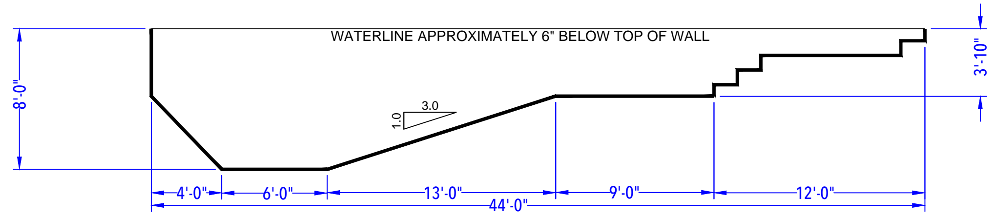
DEPTH DETAIL
