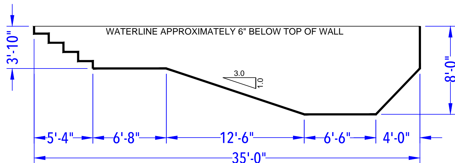
DEPTH DETAIL
