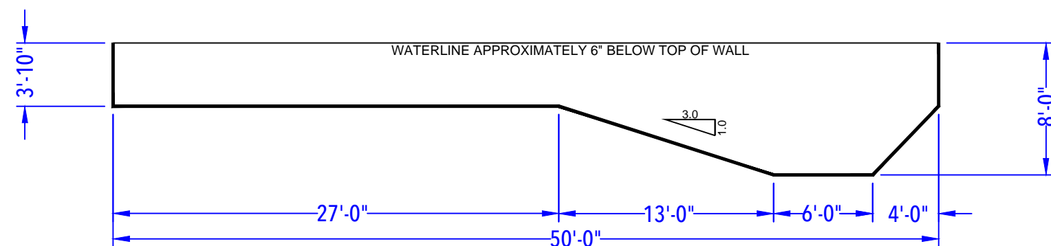
DEPTH DETAIL
