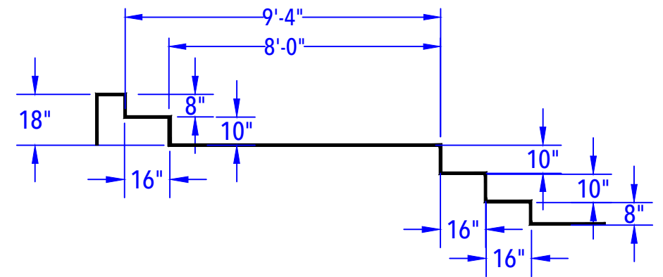
ENTRY STEP DETAIL (After Concrete & Liner) N.T.S.
