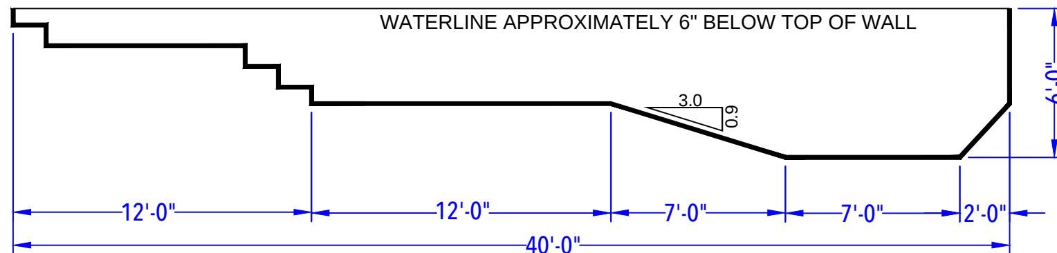
DEPTH DETAIL
