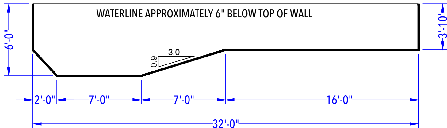
DEPTH DETAIL
