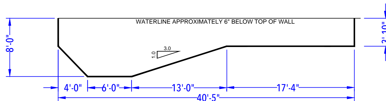
DEPTH DETAIL
