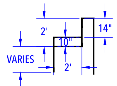
DEEP END BENCH & STEP OUT DETAIL (After Concrete & Liner) N.T.S.
