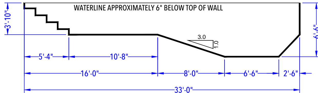
DEPTH DETAIL
