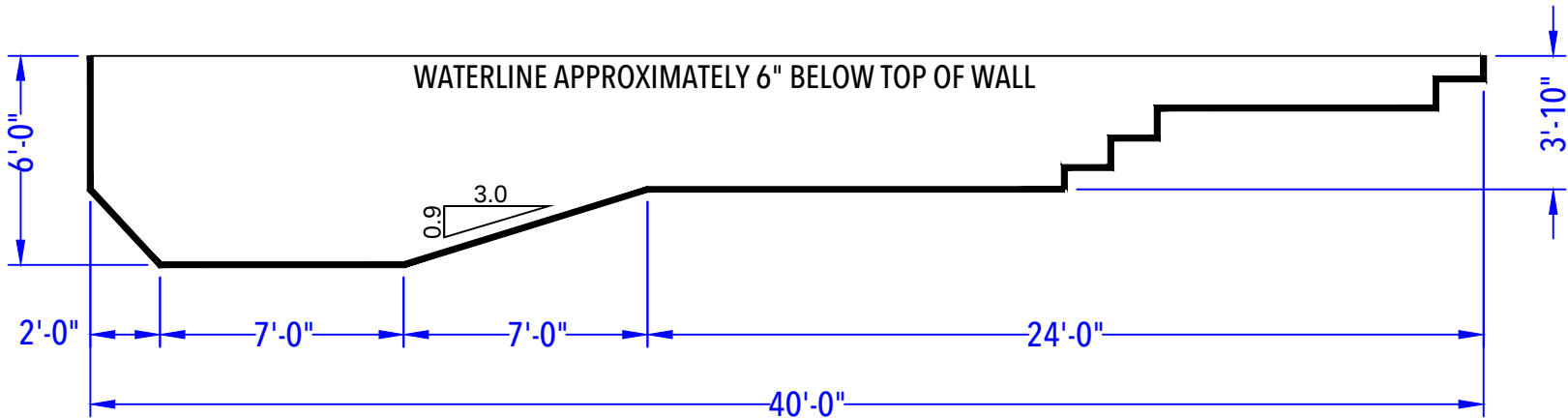
DEPTH DETAIL
