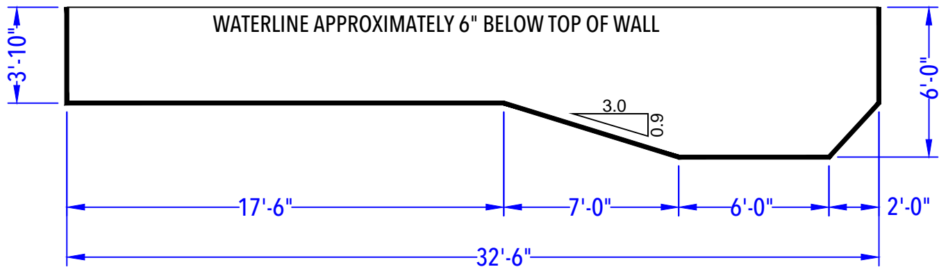
DEPTH DETAIL
