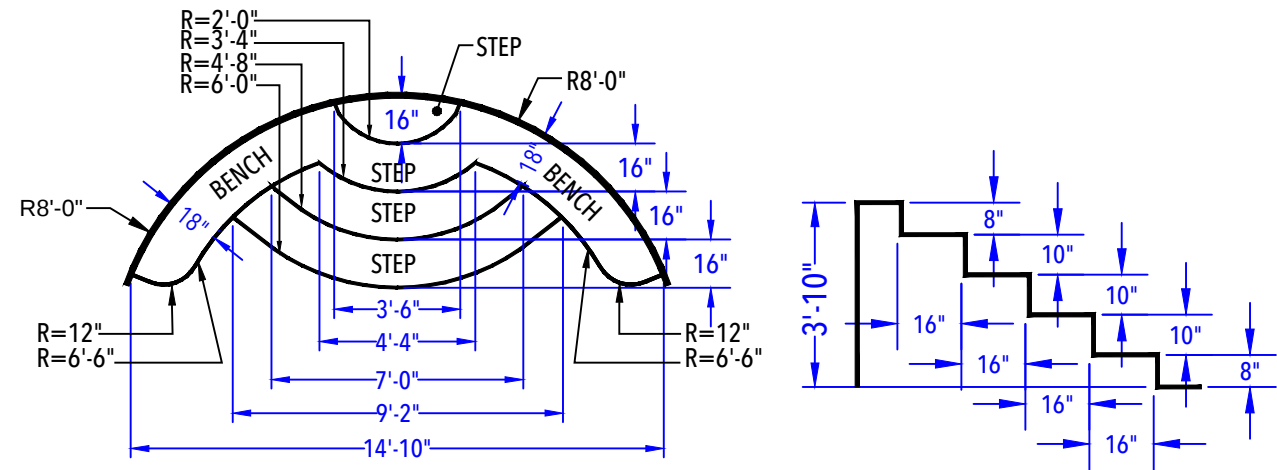
ENTRY STEP DETAIL (After Concrete & Liner) N.T.S.
