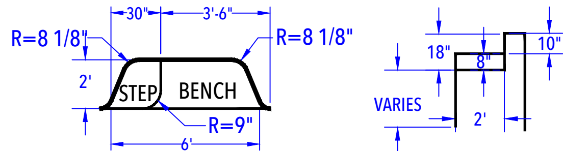
DEEP END BENCH & STEP OUT DETAIL (After Concrete & Liner) N.T.S.
