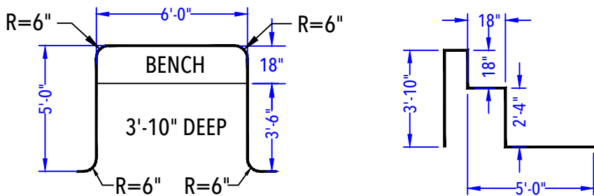
DEEP END BENCH AT GROTTA DETAIL (After Concrete & Liner) N.T.S.
