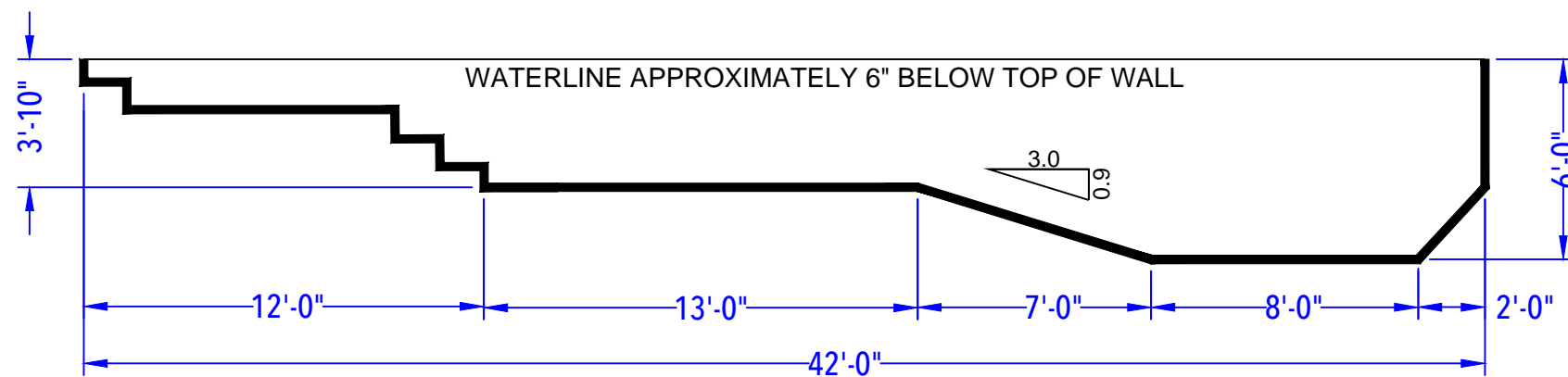
DEPTH DETAIL
