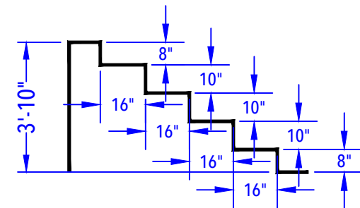
CORNER ENTRY STEP AND SHALLOW END BENCH DETAIL (After Concrete & Liner) N.T.S.
