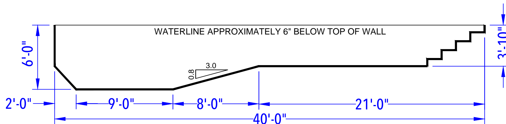
DEPTH DETAIL
