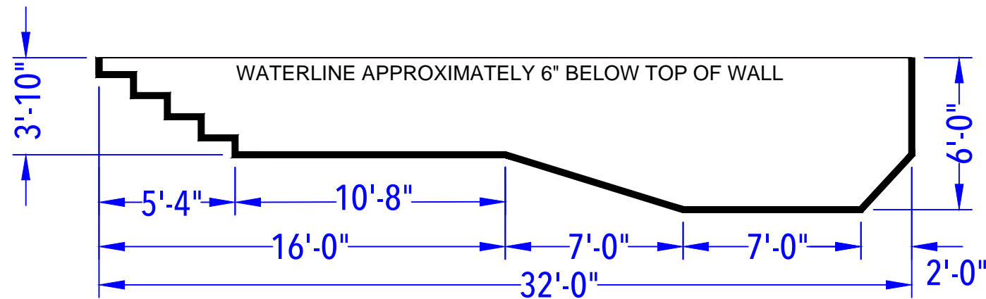
DEPTH DETAIL
