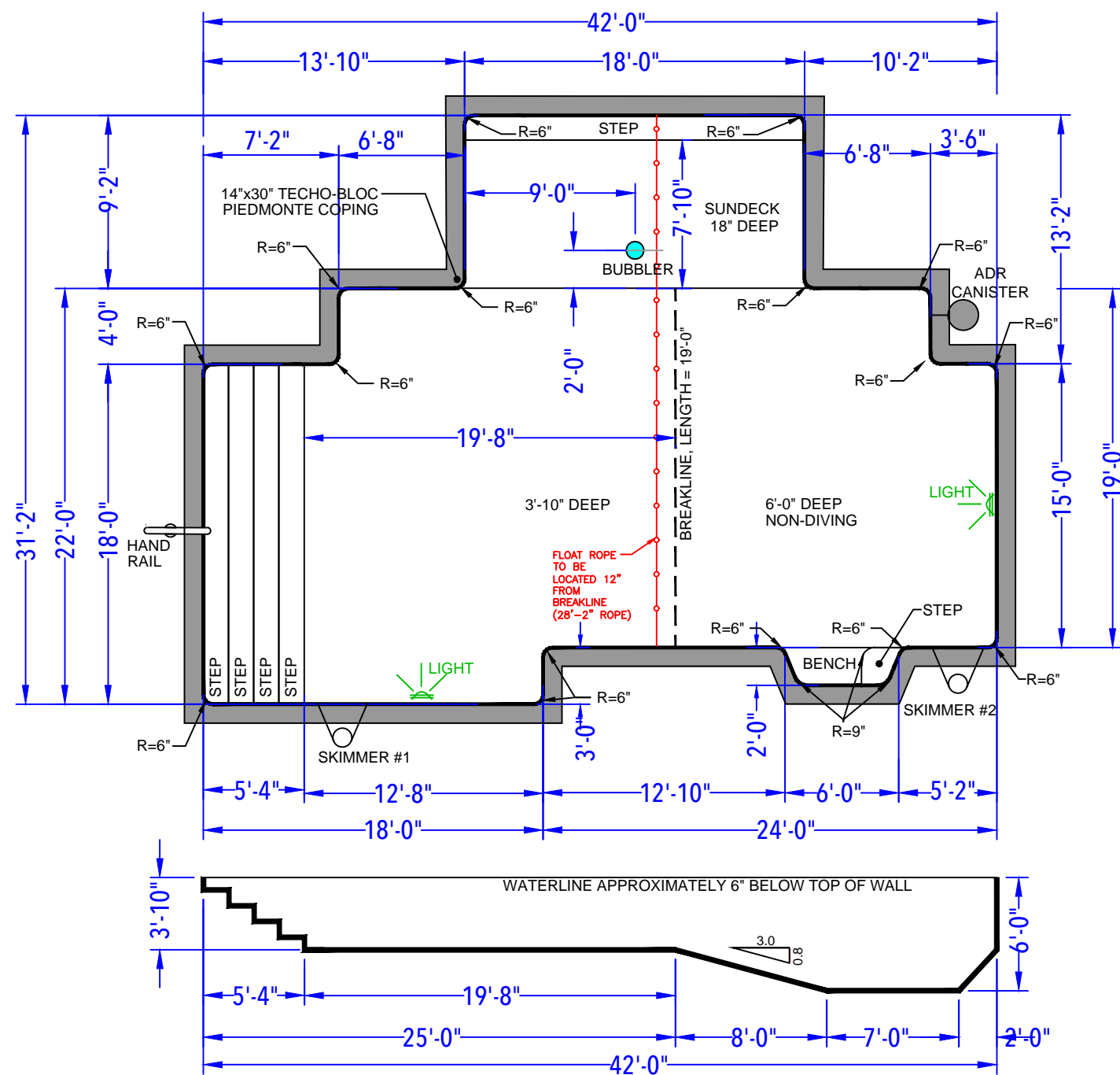
DEPTH DETAIL
