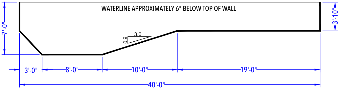
DEPTH DETAIL
