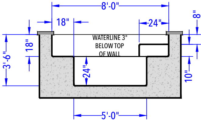
SPA PLAN & ELEVATION VIEW (After Concrete & Plaster)
