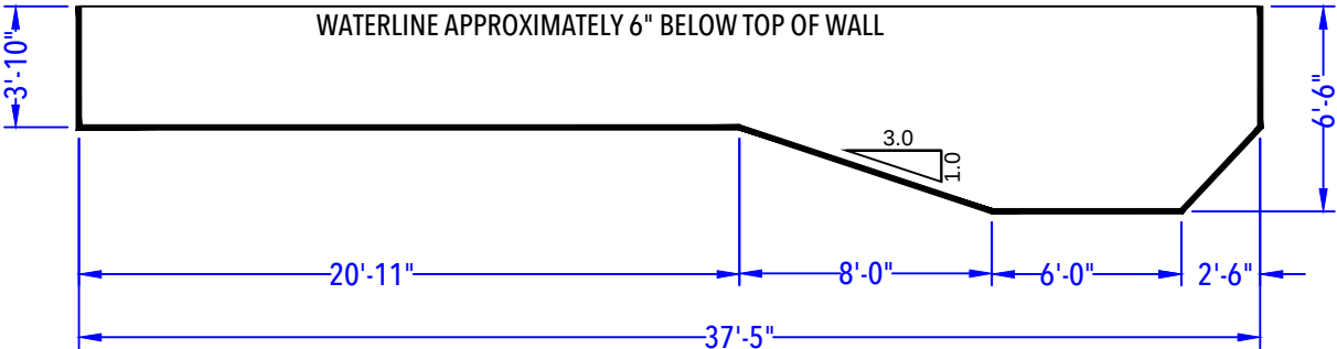
DEPTH DETAIL
