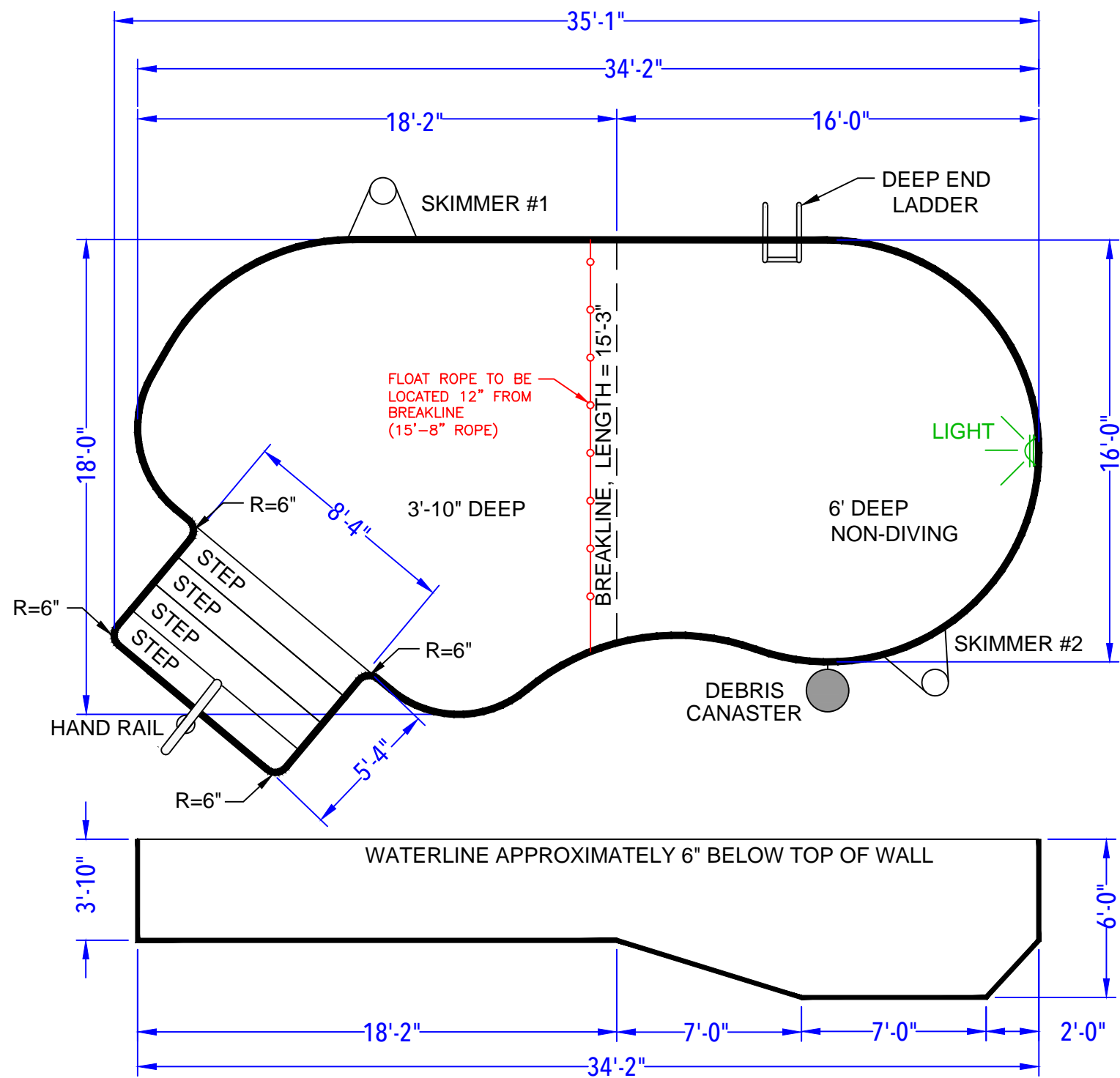
DEPTH DETAIL
