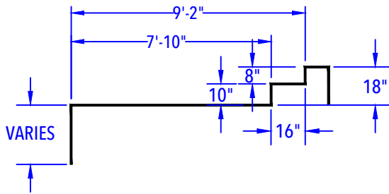
SIDE SUN DECK DETAIL (After Concrete & Liner) N.T.S.
