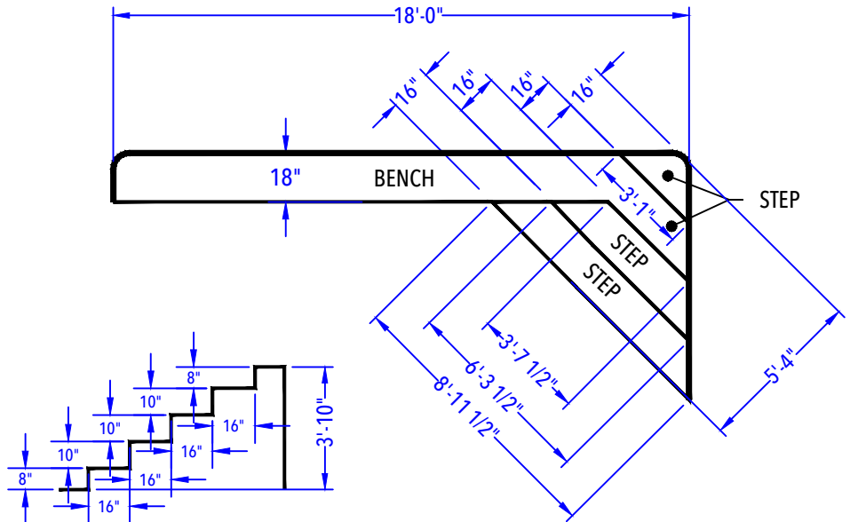
ENTRY STEP DETAIL (After Concrete & Liner) N.T.S.
