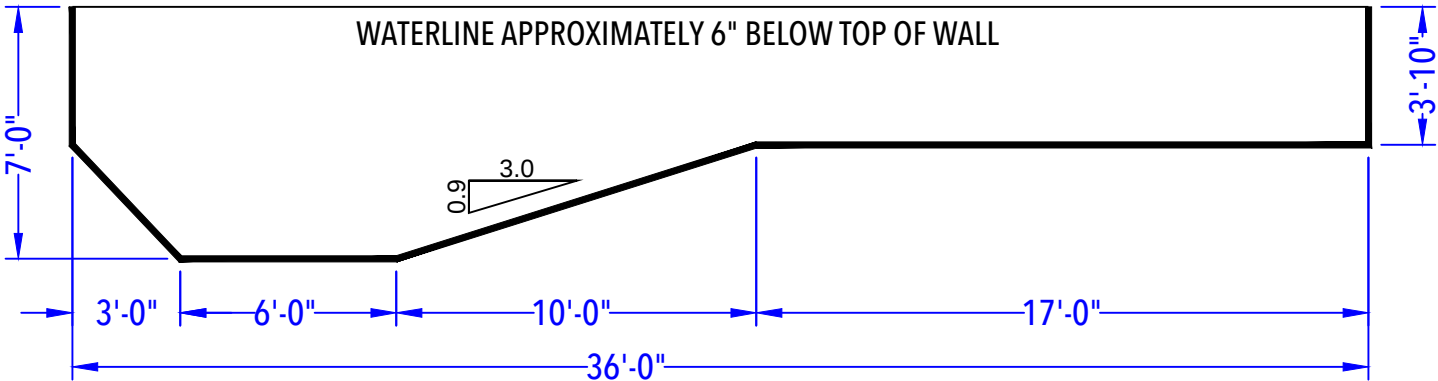
DEPTH DETAIL
