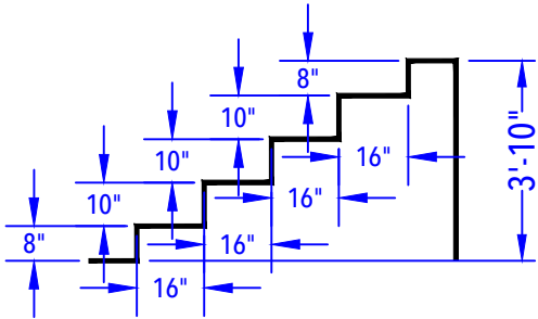
CORNER ENTRY STEP DETAIL (After Concrete & Liner) N.T.S.
