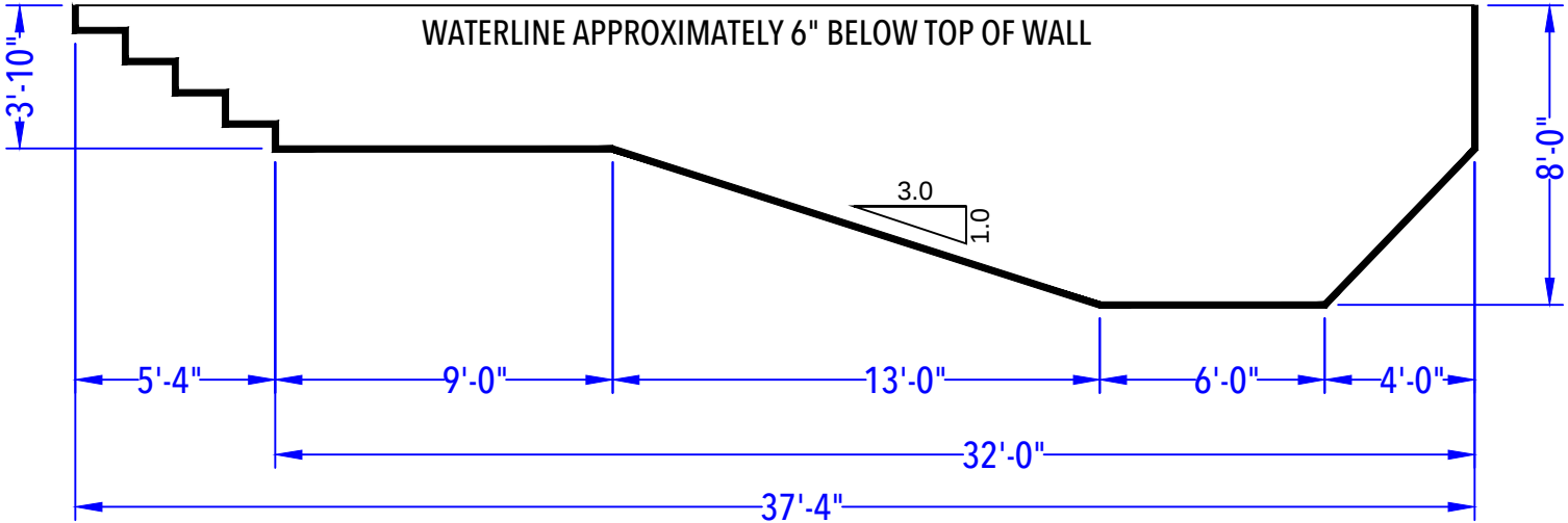
DEPTH DETAIL
