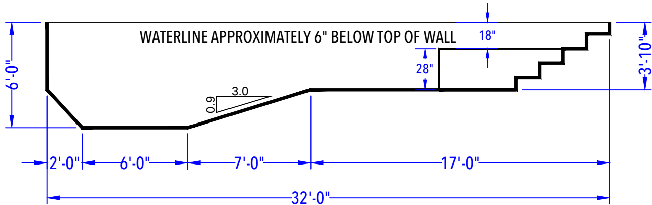
DEPTH DETAIL
