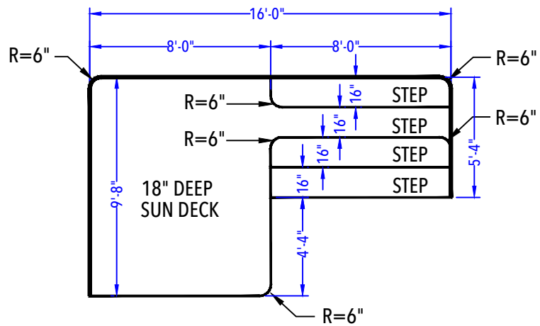
SUN DECK & ENTRY STEP DETAIL (After Concrete & Liner) N.T.S.
