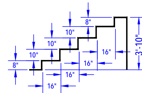
ENTRY STEP & BENCH DETAIL (After Concrete & Liner) N.T.S.
