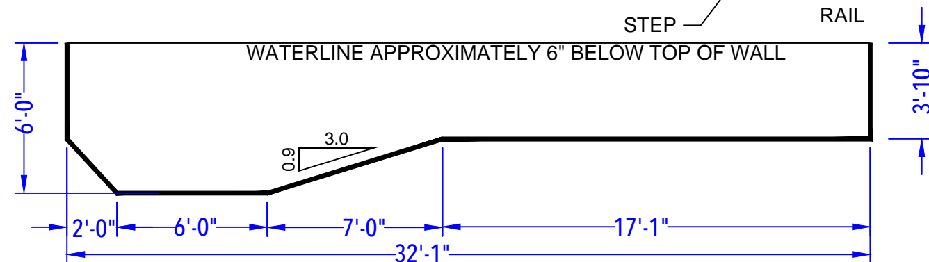
DEPTH DETAIL
