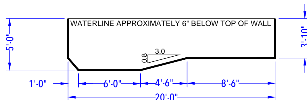
DEPTH DETAIL
