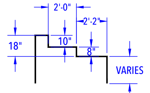
DEEP END BENCH & STEP OUT DETAIL (After Concrete & Liner) N.T.S.
