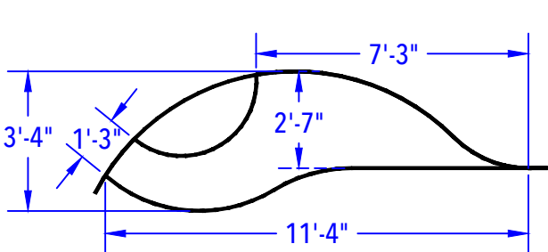
DEEP END BENCH & STEP OUT DETAIL (After Concrete & Liner) N.T.S.
