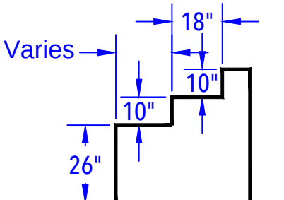
DEEP END BENCH & STEP OUT DETAIL (After Concrete & Liner) N.T.S.
