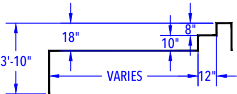
SIDE SUN DECK DETAIL (After Concrete & Liner) N.T.S.
