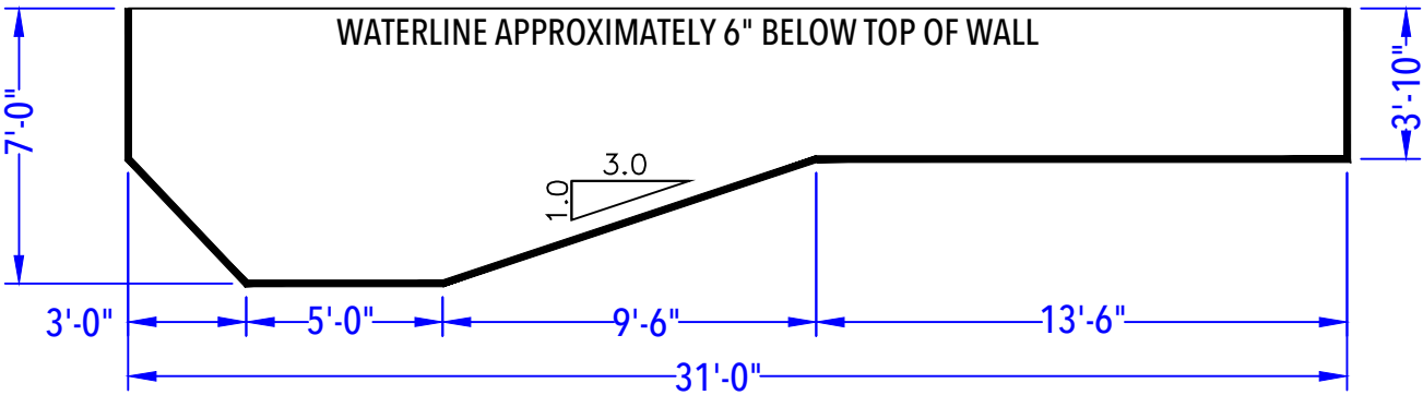
DEPTH DETAIL
