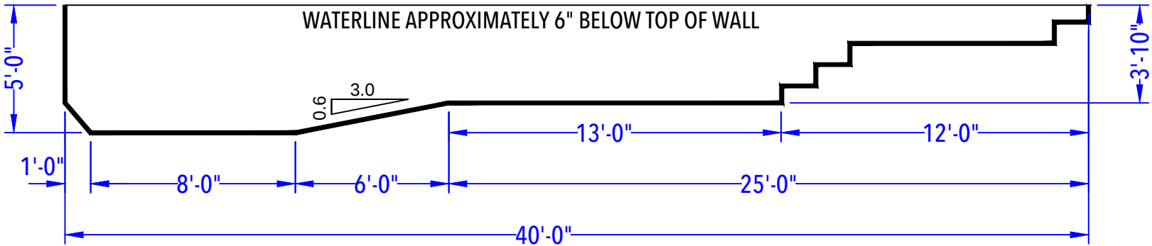
DEPTH DETAIL
