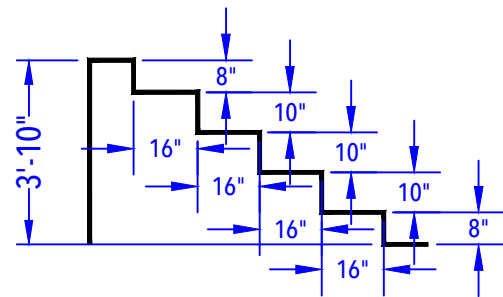
CORNER STEP & BENCH DETAIL (After Concrete & Liner) N.T.S.
