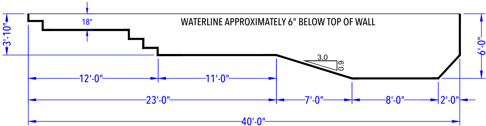
DEPTH DETAIL
