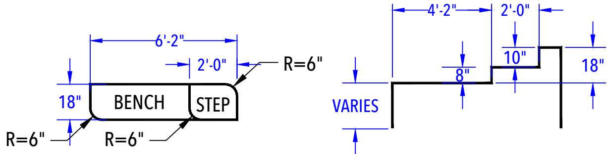
DEEP END BENCH & STEP OUT DETAIL (After Concrete & Liner) N.T.S.
