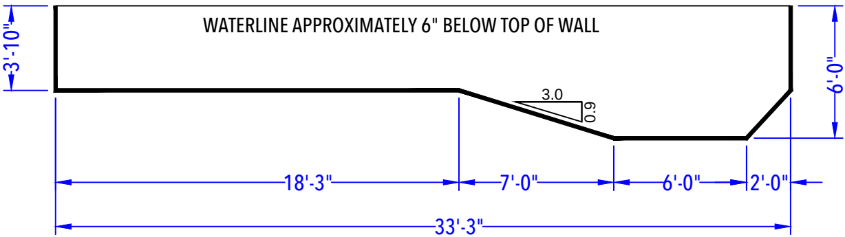
DEPTH DETAIL
