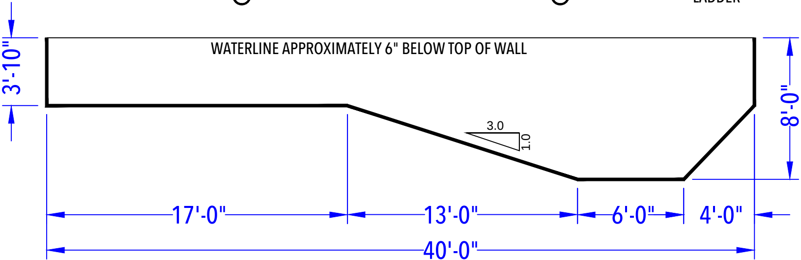
DEPTH DETAIL
