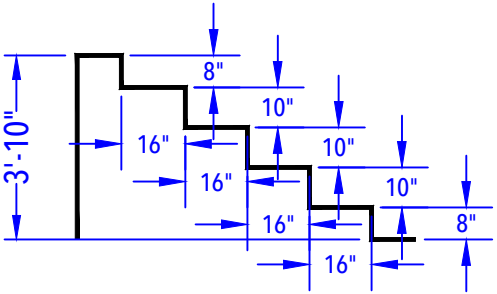
ENTRY CORNER STEP DETAIL (After Concrete & Liner) N.T.S.
