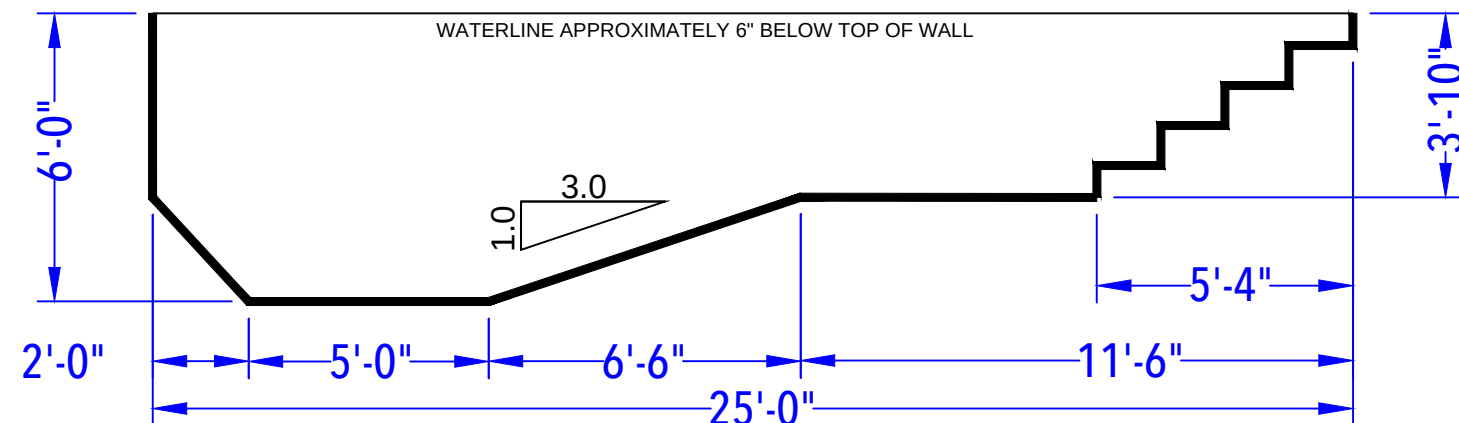
DEPTH DETAIL
