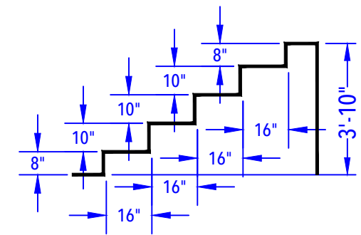
STEP DETAIL (After Concrete & Liner) N.T.S.
