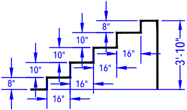
ENTRY STEP DETAIL (After Concrete & Liner) N.T.S.
